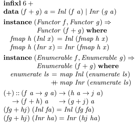
Figure 6. Species sum
