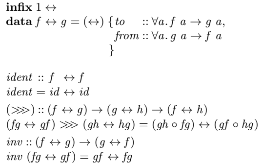
Figure 7. Isomorphisms
