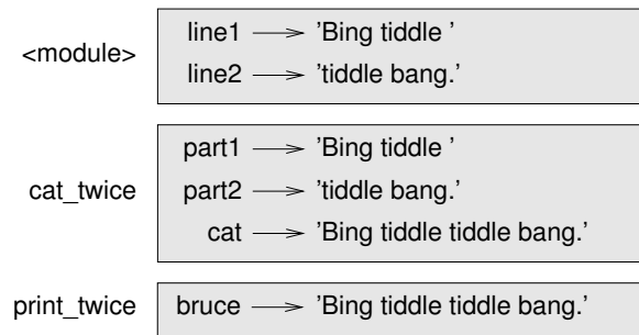
Figure 5.1: Stack diagram.
